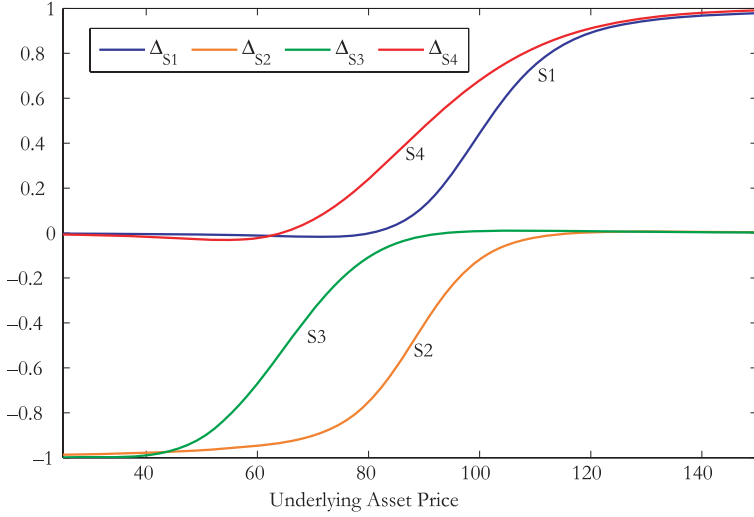
FIGURE 4.1. Deltas with respect to all four underlying asset prices.
